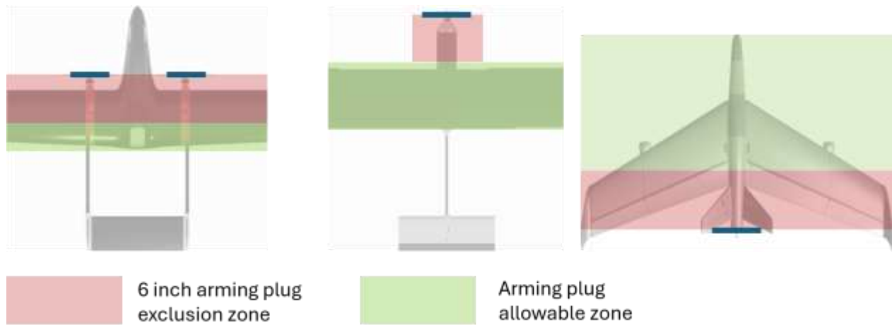
Figure 3. Arming Plug Location Requirements.
