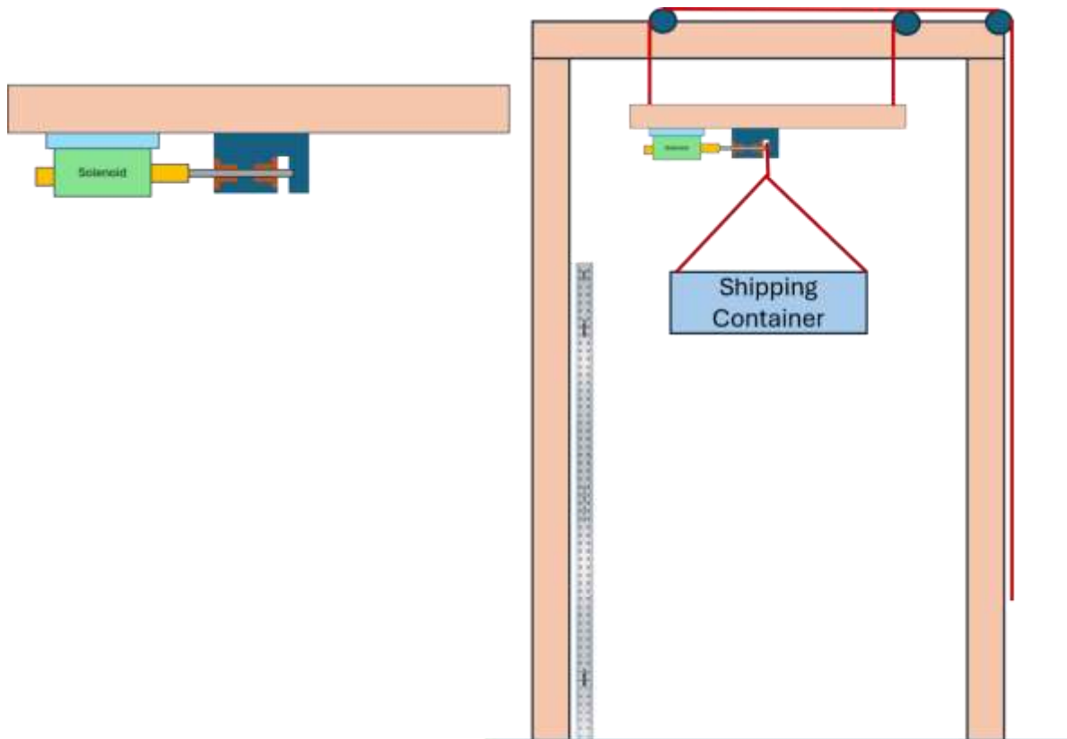
Figure 6. Adjustable Height Quick Release Mechanism.
