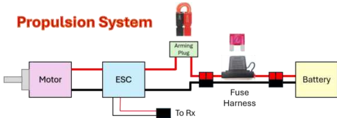
Figure 4. Propulsion System Wiring Requirements.
